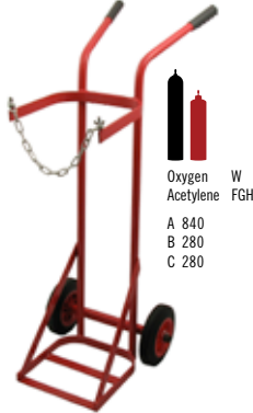
Part No. 1271 Single Oxygen/Acetylene Cylinder Trolley
