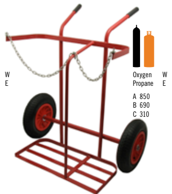
Part No. 1275 Oxygen/Propane Cylinder Trolley 16" Pneumatic Tyres
