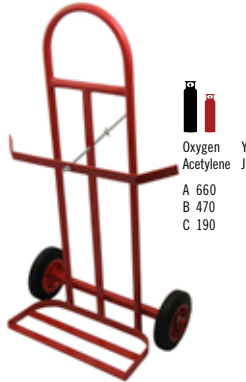
Part No. 1279 Oxygen/Acetylene Y-Type Cylinder Trolley
