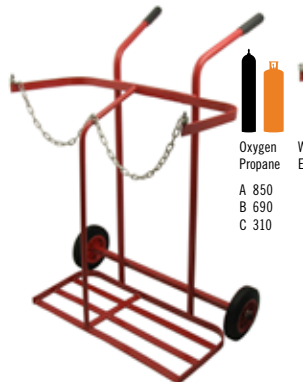
Part No. 1268 Oxygen/Propane Cylinder Trolley
