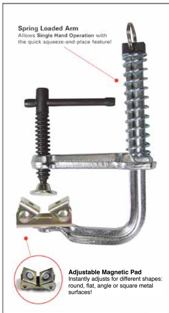
Stays in place while you tighten. Ideal for One-Handed clamping:
